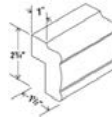
Light Rail Moulding Length – 96" Depth – 1 1/2" Height – 2 1/4"
