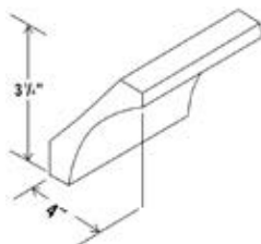
Cove Crown Moulding Length – 96" Depth – 4" Height – 3 1/4"
