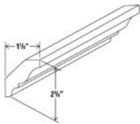
Crown Moulding Length – 96" Depth – 5/8" Height – 2 3/4"
