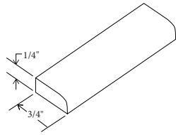
Scribe Moulding Length - 96" Depth - 3/4" Height - 1/4"
