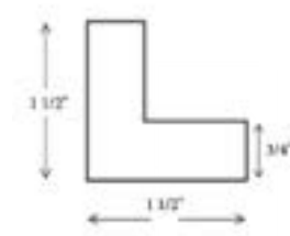
L-Shape Moulding Length - 96" Depth - 1 1/2" Height - 1 1/2"
