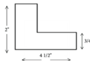
Raiser Moulding Length - 96" Depth - 2" Height - 4 1/2"
